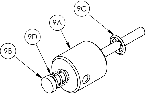
ITEM 9, TRANSFER BAR ASSY
